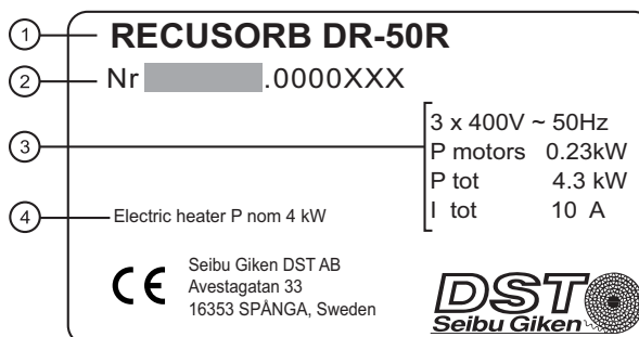
IMAGE 1: Plaque signalétique
