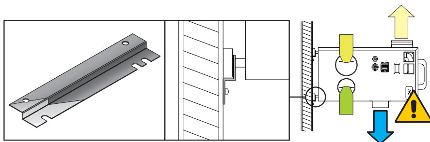
FIGURE 11: Bracket for wall mount
