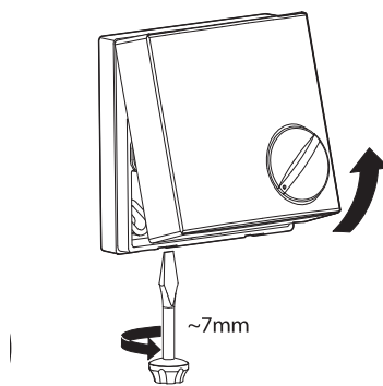
FIGUR 14: Lucka
