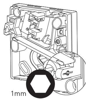
IMAGE 15: Vis de calibrage
