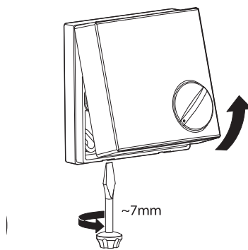
FIGURE 15: Lid
