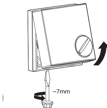
FIGUR 15: Lucka
