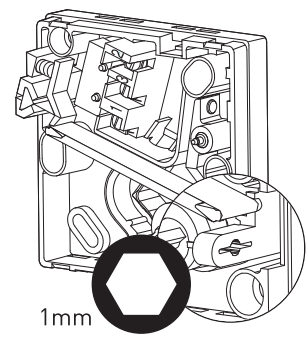
IMAGE 16: Vis de calibrage
